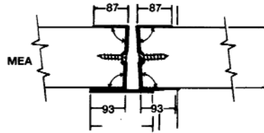
Metal Edges (pair) with Astragal for swinging doors
