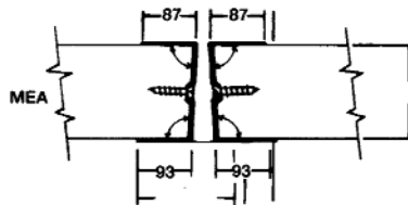
Metal Edges (pair) for swinging doors
