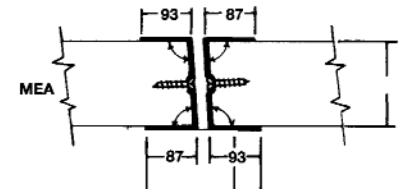
Metal Edges (pair) for double egress doors
