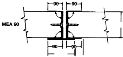
Metal Edges (pair) with Astragal for 90° doors
