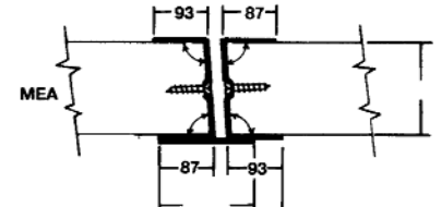
Metal Edges (pair) with Astragal for double egress doors
