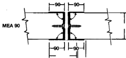
Metal Edges (pair) for 90° doors
